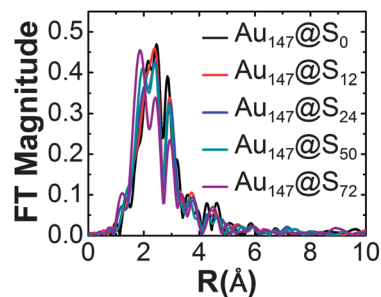
Fig. 2 A comparison of the EXAFS data in R -space for \text{Au}_{147}@\text{S}_n DENs.
