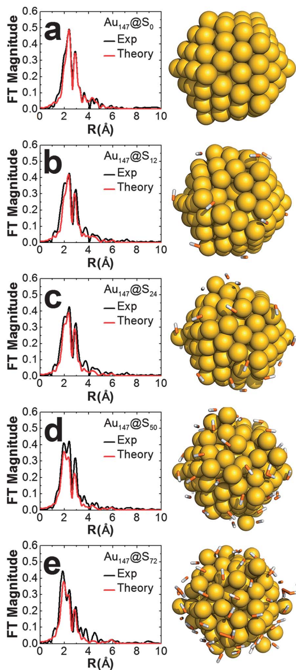
Fig. 6 Left side. Comparison of experimentally and theoretically derived EXAFS data in R -space: (a) \text{Au}_{147}@\text{S}_0 , (b) \text{Au}_{147}@\text{S}_{12} , (c) \text{Au}_{147}@\text{S}_{24} , (d) \text{Au}_{147}@\text{S}_{50} , (e) \text{Au}_{147}@\text{S}_{72} . Right side: Representative snapshots of the DFT-MD trajectories taken from the portion of the simulations used to calculate the theoretical EXAFS signals and PDFs.
