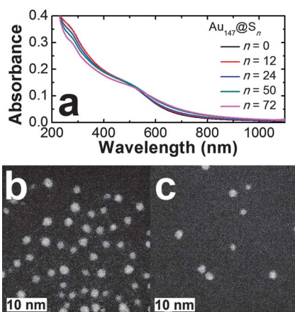
Fig. 1 (a) UV-vis spectra of \text{Au}_{147}@\text{S}_n DENs ( n = 0, 12, 24, 50, and 72 ). Representative STEM images of (b) \text{Au}_{147}@\text{S}_0 and (c) \text{Au}_{147}@\text{S}_{72} DENs extracted from the pellet used for the EXAFS experiments following analysis. White boxes represent the 10 nm scale bar.
